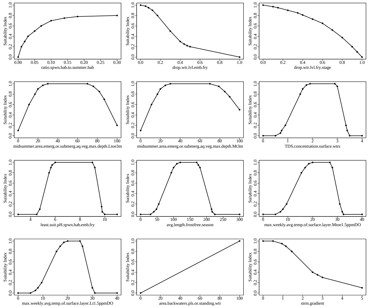
Figure 1. Suitability index graphs for variables included in the northernpikeRivVegB model in ecoest.
